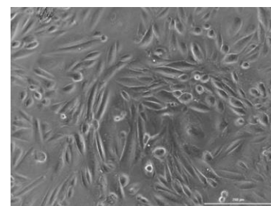
Cell morphology. Cells in culture were fixed in situ and photographed using a phase contrast microscope. (Bar: 200µm)
